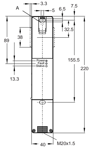
Connector type D41G-□□D□-N2
