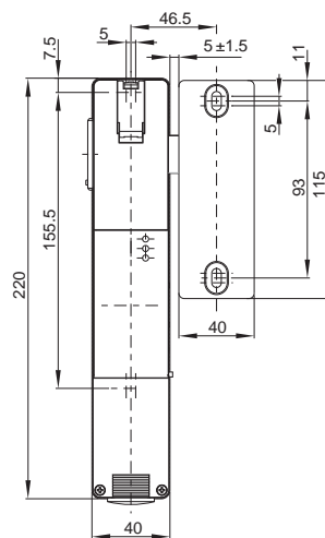
For right (D41G-A1R)
