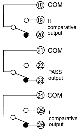
K3NR with 5 Relay Output Boards, K31-C5
