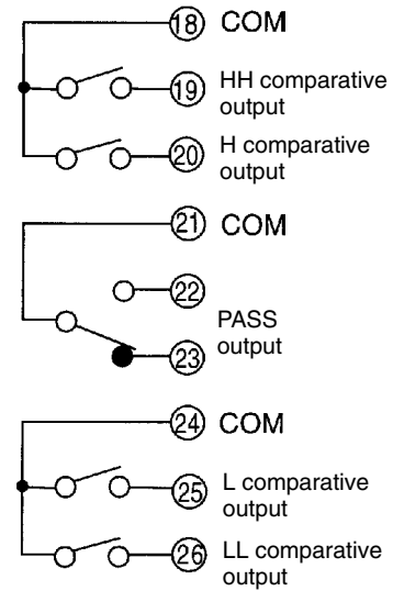
K3NR with 5 Relay Output Boards, K31-C5
