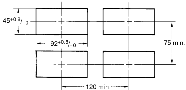
Panel Cutout
