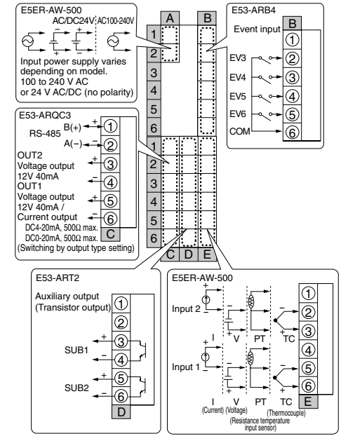
E5ER-QT3DW-FLK (2-input type)
