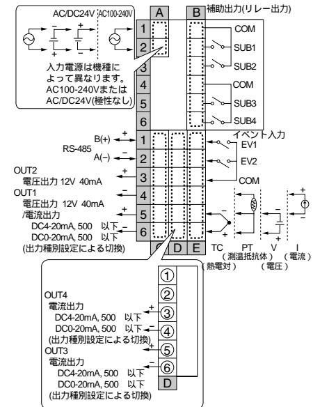
E5ER-QC43B-FLK
