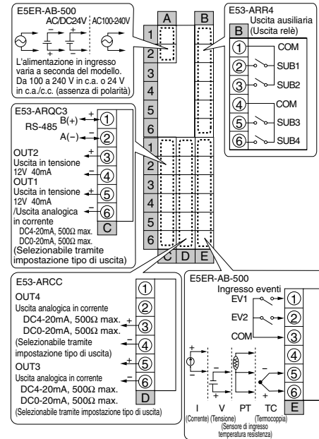
E5ER-QC43B-FLK
