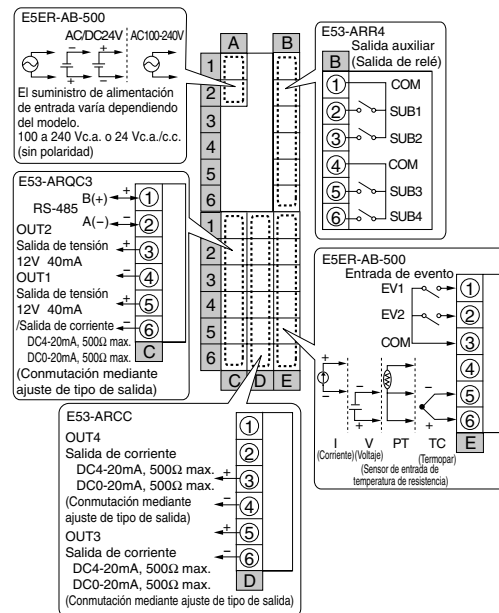
E5ER-QC43B-FLK
